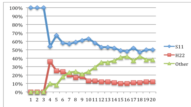
Figure 5. Betweenness centrality of early adopter teams (S11, H22) decreases as others increase.
