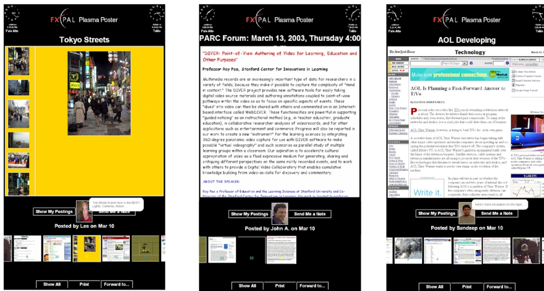
Figure 3: Examples from the “PosterShow” Interface: posted images, text and a URL. Author comments appear in speech bubbles by their photographs. Other content appears as thumbnails below the currently displayed ‘main’ posting. Bottom buttons are for overviews, printing and messaging.
