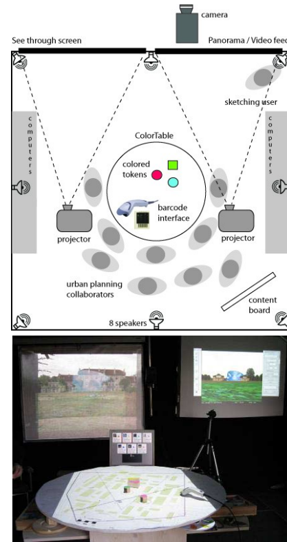
Figure 6: The technical setup inside the MR Tent is centered around the two projection walls and the ColorTable
