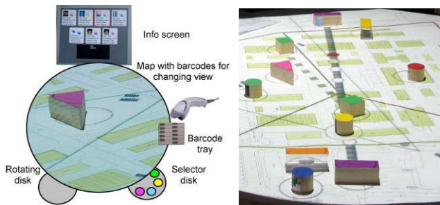
Figure 7: Setup of the tangible table and example of a composed scene including objects, rows, land use, roads and flows (top view)
